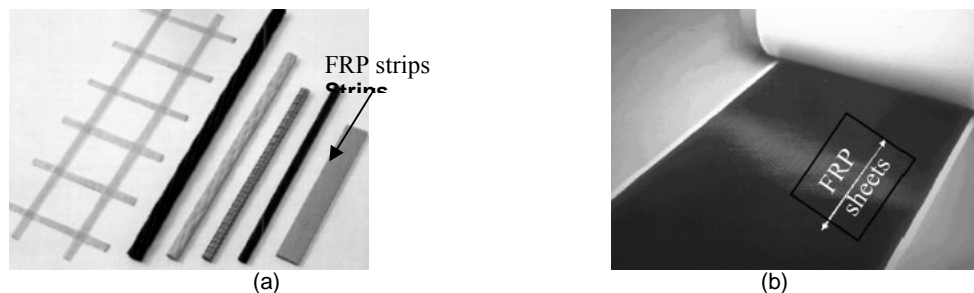
Figure 1. FRP products for structural rehabilitation, (a) FRP strips and (b) FRP sheets (Rizkalla et al. 2003).
