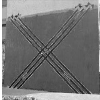
Figure 4. Seismic retrofitting of masonry shear wall with GFRP sheets (Motavalli & Czaderski, 2007)
